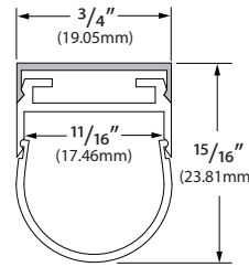
TPL-AL-CHAN-1A-8* AL Series Aluminum Channel with Mounting Carrier Base. Available in 8 ft standard lengths.
