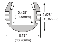
NOVA NOVA Anodized Aluminum Extrusion, available in 6.5' lengths
