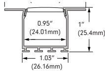
NOYS NOYES Anodized Aluminum Extrusion, available in 6.5' lengths
