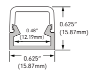
INF INFINITY PC extrusion, available in 8' length
