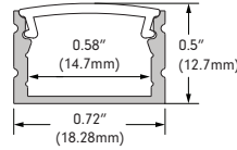
MOFFT MOFFETT Anodized Aluminum Extrusion, available in 6.5' lengths
