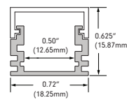
ASTR ASTORIA Anodized aluminum extrusion available in 6.5' length
