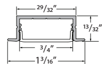
WRNR-CHAN-SLV-6.5 Anodized Aluminum Extrusion, available in 6.5' lengths
