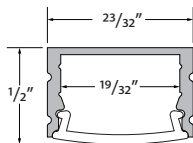
MOFT-CHAN-SLV-6.5 Anodized Aluminum Extrusion, available in 6.5' lengths
