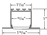
NOYS-CHAN-SLV-6.5 Anodized Aluminum Extrusion, available in 6.5' lengths
