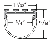
DOME-CHAN-SLV-6.5 Anodized Aluminum Extrusion, available in 6.5' lengths
