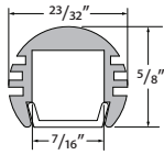
NOVA-CHAN-SLV-6.5 Anodized Aluminum Extrusion, available in 6.5' lengths
