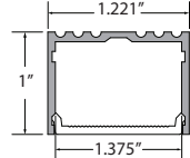
ALTN-CHAN-SLV-6.5 Anodized Aluminum Extrusion, available in 6.5' lengths
