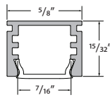
CARU-CHAN-SLV-6.5 Anodized aluminum extrusion, available in 6.5' lengths
