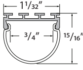
DOME-CHAN-SLV-6.5 Anodized Aluminum Extrusion, available in 6.5' lengths
