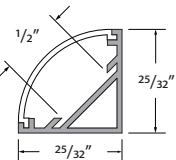
MRSL-CHAN-SLV-6.5 Anodized aluminum extrusion available in 6.5' length
