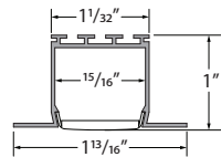
NOYS-CHAN-SLV-6.5 Anodized Aluminum Extrusion, available in 6.5' lengths
