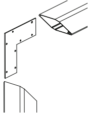
AC-90 Flat 90° (Standard) Internal 90° Bracket
