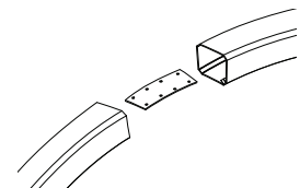
AC-RADIUS Internal Bracket
