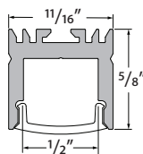
VALN-CHAN-SLV-6.5 Anodized Aluminum Extrusion, available in 6.5' lengths
