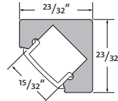
DYER-CHAN-SLV-6.5 Anodized Aluminum Extrusion, available in 6.5' lengths
