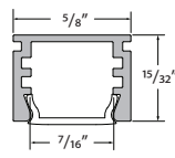
CARU-CHAN-SLV-6.5 Anodized aluminum extrusion, available in 6.5' lengths
