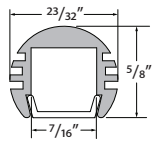
NOVA-CHAN-SLV-6.5 Anodized Aluminum Extrusion, available in 6.5' lengths
