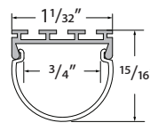
DOME-CHAN-SLV-6.5 Anodized Aluminum Extrusion, available in 6.5' lengths
