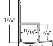
EDGE-CHAN-SLV-6.5 Anodized Aluminum Extrusion, available in 6.5' lengths
